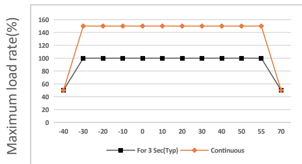
Environmental Temperature(°C)
