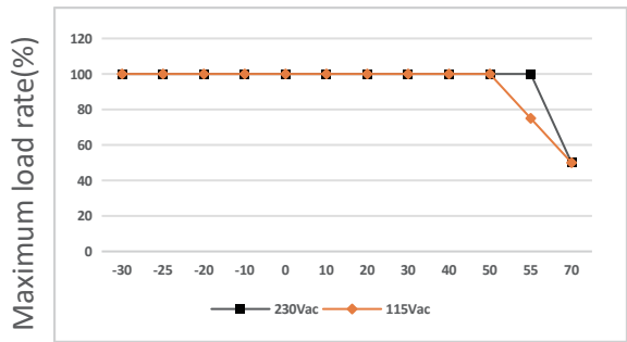
Environmental Temperature(°C)
