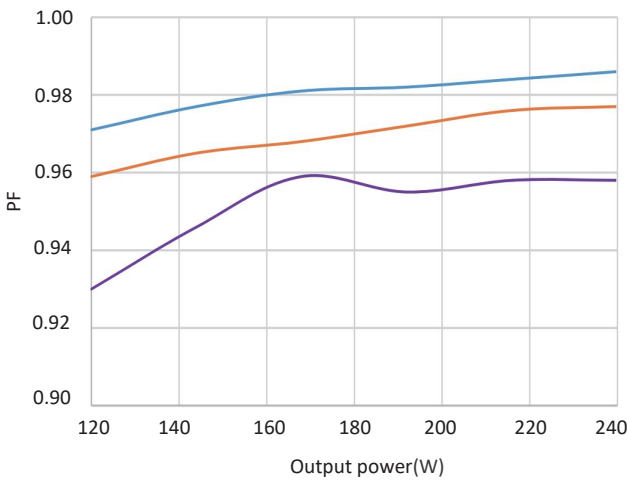
PF vs Output power
