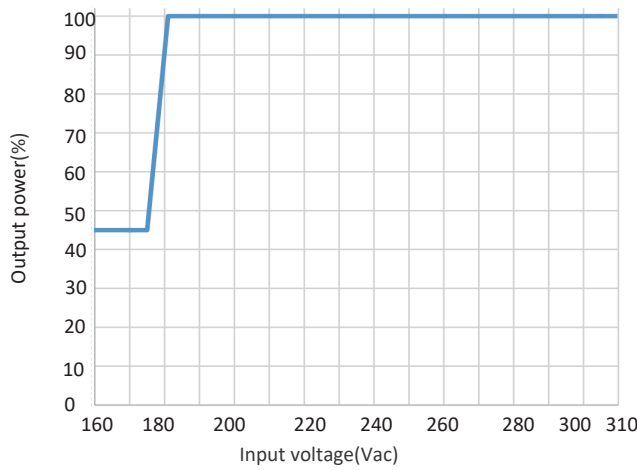
Output power VS Input voltage
