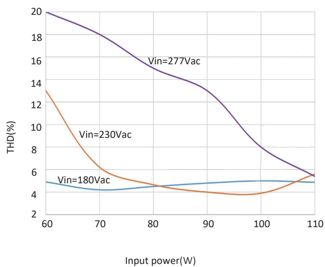
THD vs Input power
