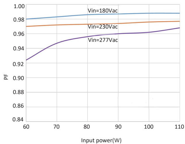
PF vs Input power
