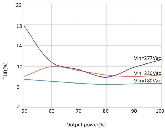
THD vs Output power
