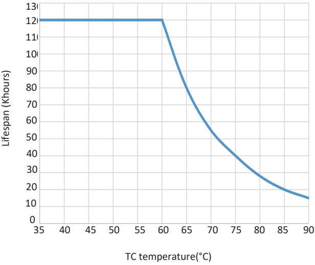
Lifespan vs TC temperature
