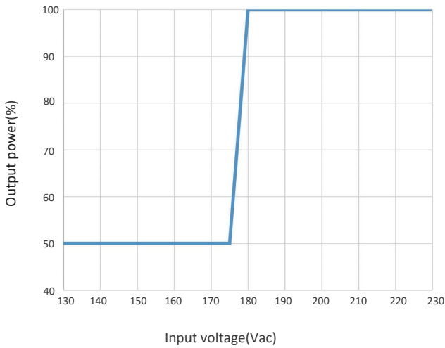
Output power VS Input voltage
