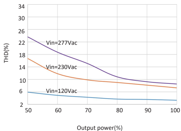
THD vs Output power
