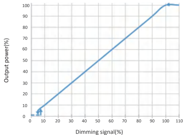
Output power VS Dimming signal
