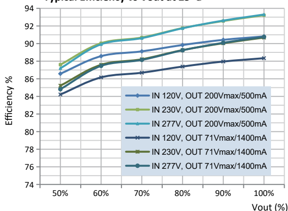
Typical Efficiency vs Vout at 25°C
