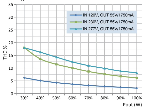
Typical THD vs Pout at 25°C
