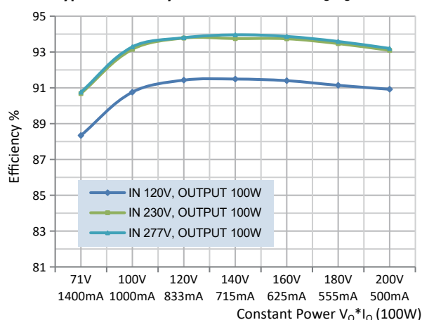
Typical Efficiency vs Constant Power V_o \cdot I_o at 25°C
