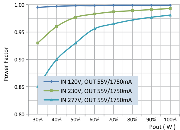
Typical PF vs Pout at 25°C
