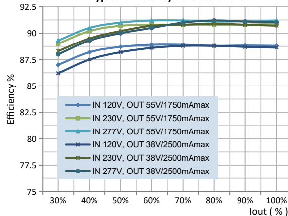
Typical Efficiency vs Iout at 25°C
