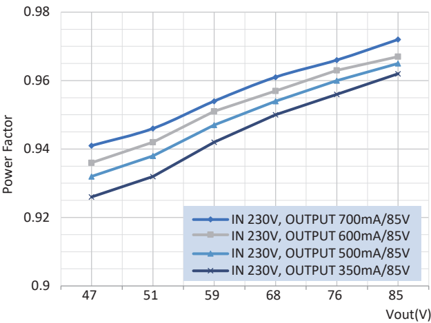
Typical PF vs Vout at 25 °C Ambient Temp
