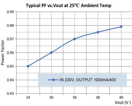
Power factor curve
