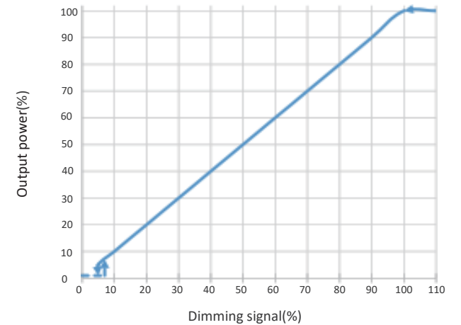
Output power VS Dimming signal
