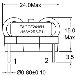
Orthographic view
