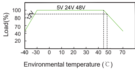
Environmental temperature derating curve
