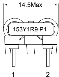
Orthographic view
