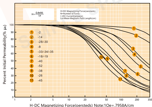
DC-Bias Curves(Typical)
