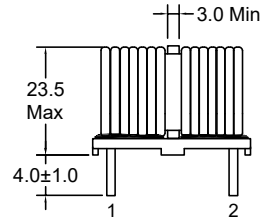
Orthographic view
