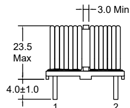
Orthographic view
