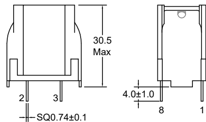
Orthographic view
