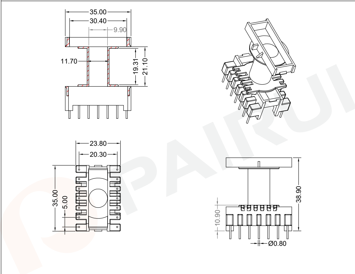
Winding data and area product for 14-pins ETD29/16/10 coil former
